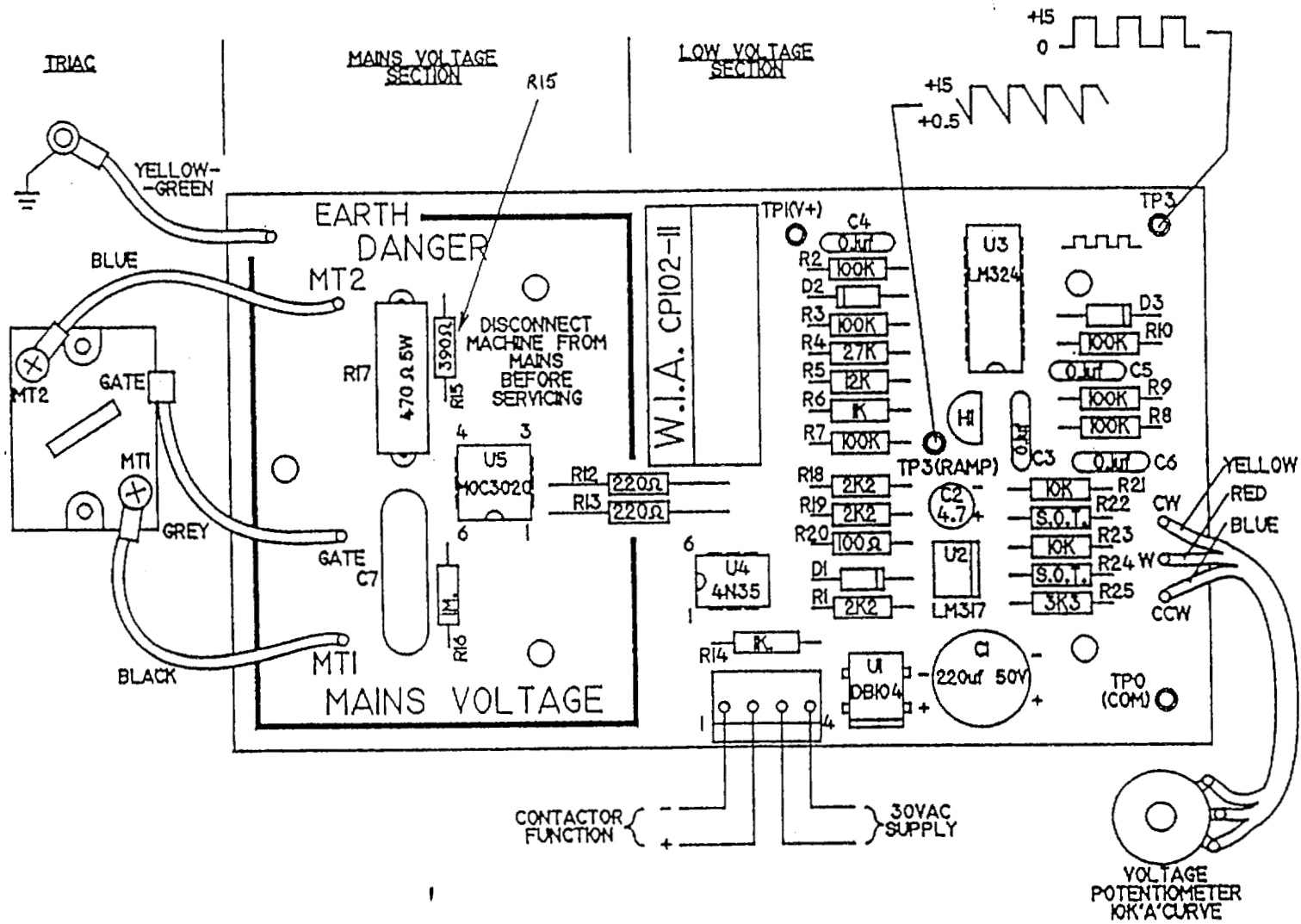
TRIAC CONTROL BOARD CP102-11
